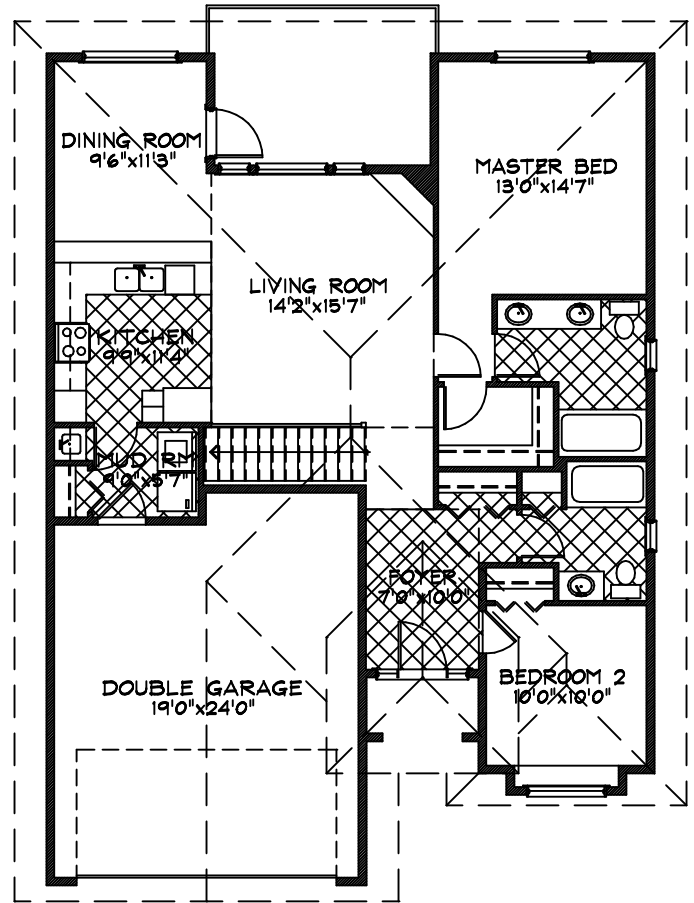
GROUND FLOOR PLAN 1232 SQ.FT.
