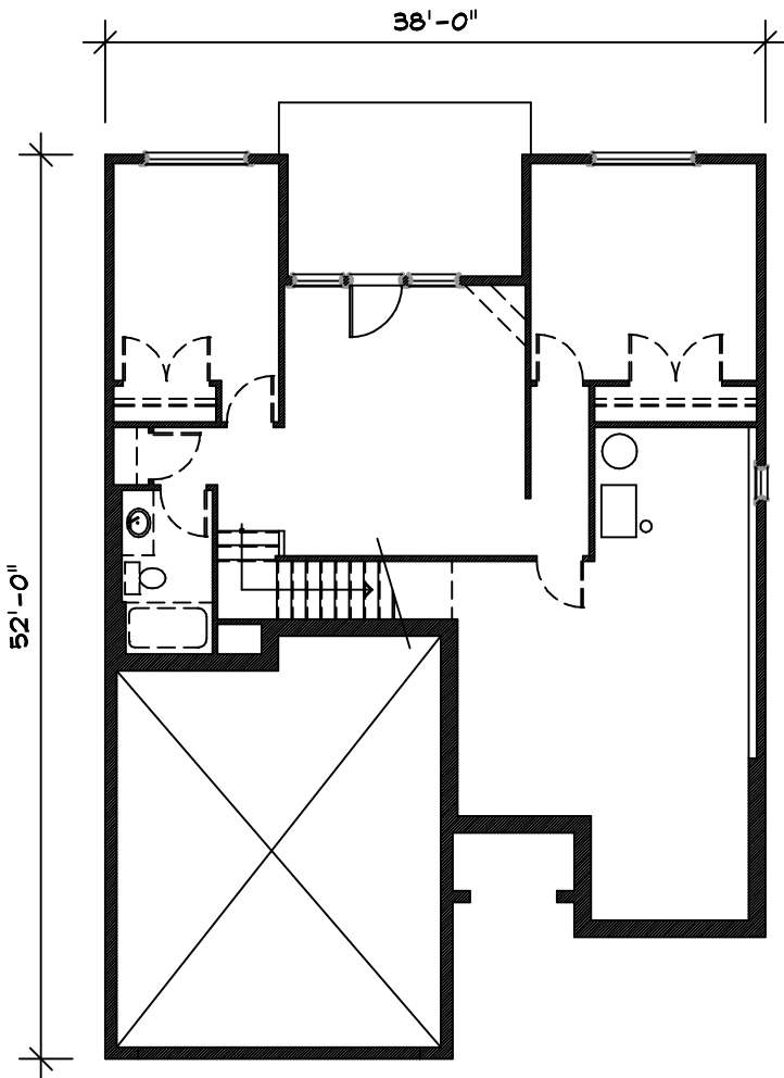
BASEMENT FLOOR PLAN UNFINISHED
