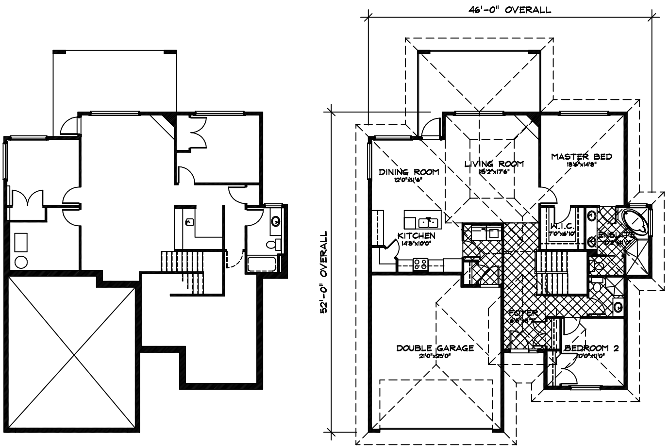
BASEMENT FLOOR PLAN UNFINISHED
